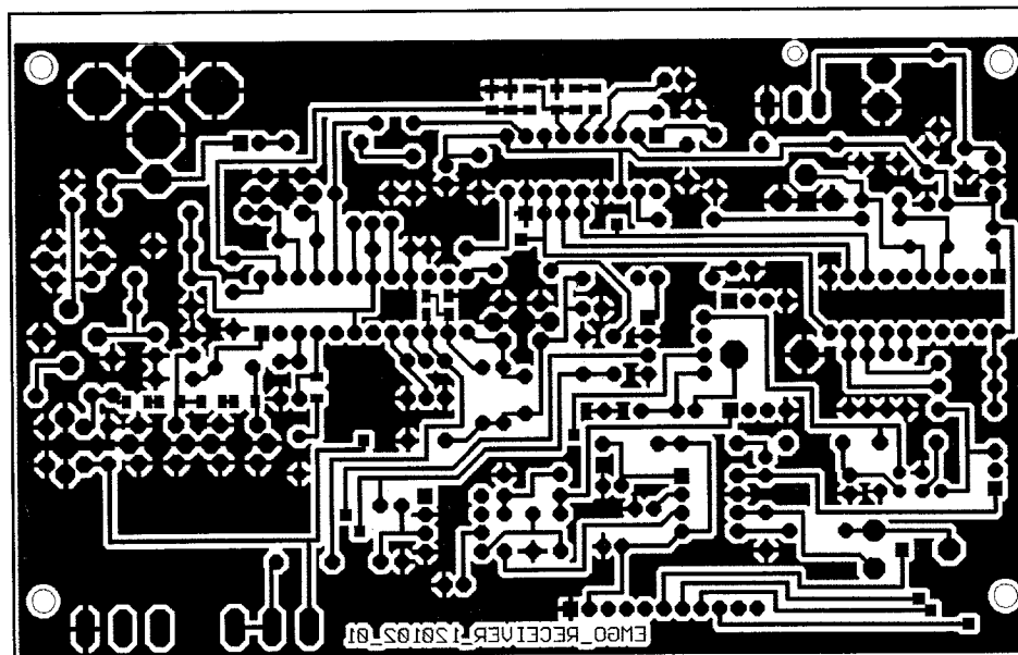
Fig 9 : Bottom side of the main receiver PCB.
